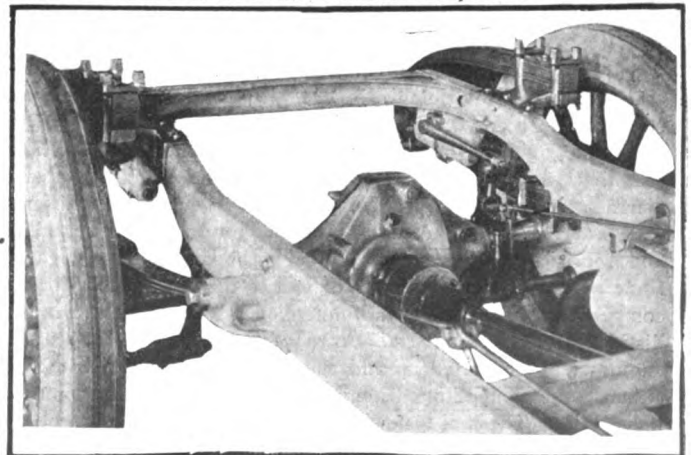
Figure IV. Thirty Special—Shaft-Drive and Level Platform Suspension
